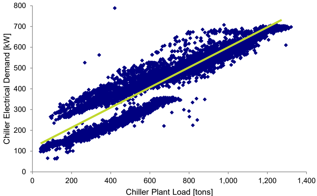
Figure 4-4: Example of Inaccurate Regression Prediction of Chiller Demand
