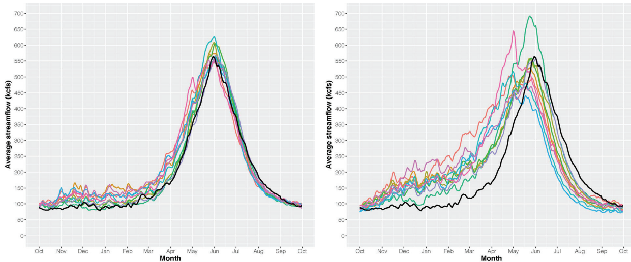
Average streamflows (in thousands of cubic feet per second) at The Dalles, Oregon. Black line is the historical average (1976–2005). Colored lines represent various climate model projections. Left is for the 2030s (2020–2049). Right is for the 2070s (2060–2089).
