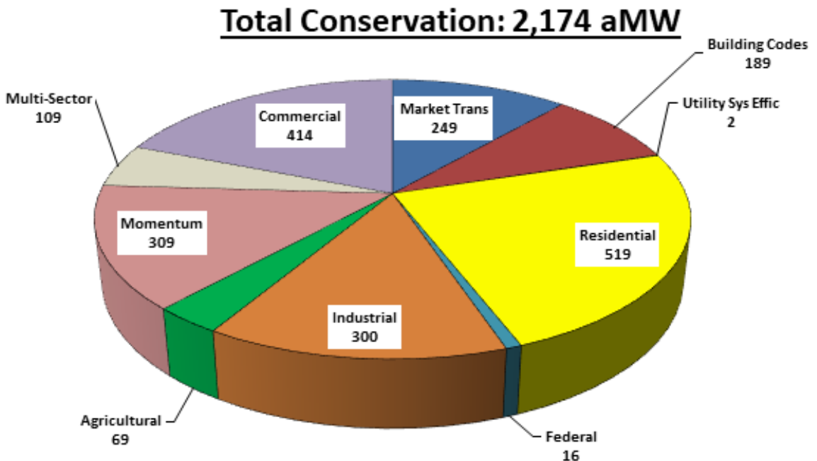
FIGURE 1. BPA's Cumulative Conservation Savings (aMW) by Sector, FY 1982-2018*
